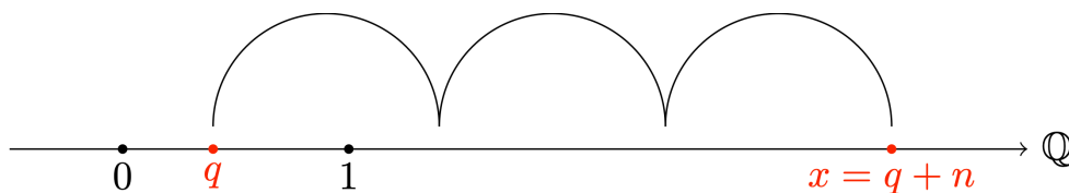
Figure 2.1: For each x \in \mathbb{Q} there exist unique q \in [0, 1) \cap \mathbb{Q} such that x = q + n . In particular [x] = [q] .
