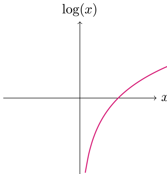
Figure 2.10: Plot of function g(x) = \log(x)
