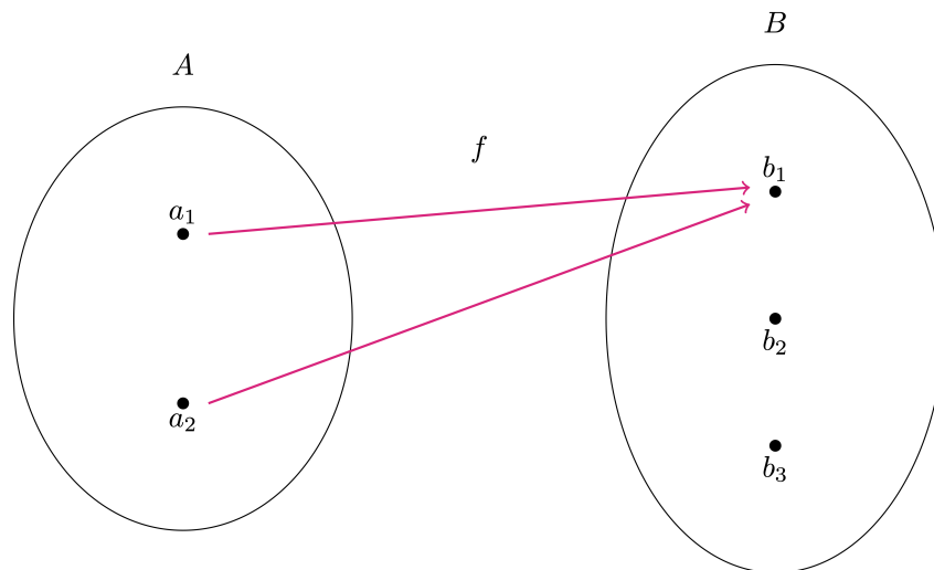
Figure 2.6: Schematic picture of the function f
