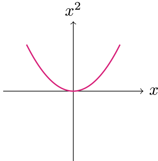
Figure 2.9: Plot of function f(x) = x^2
