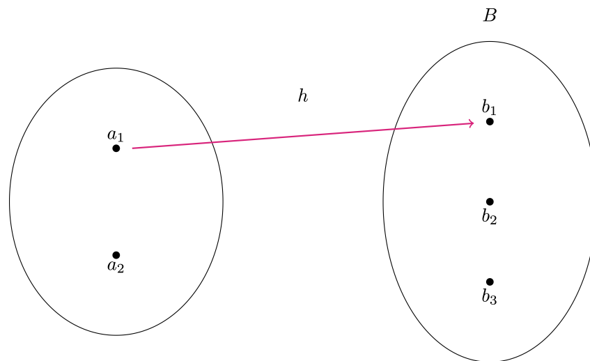
Figure 2.8: Schematic picture of the function h
