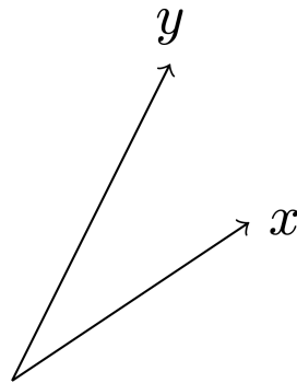
Figure 2.15: Vectors x and y
