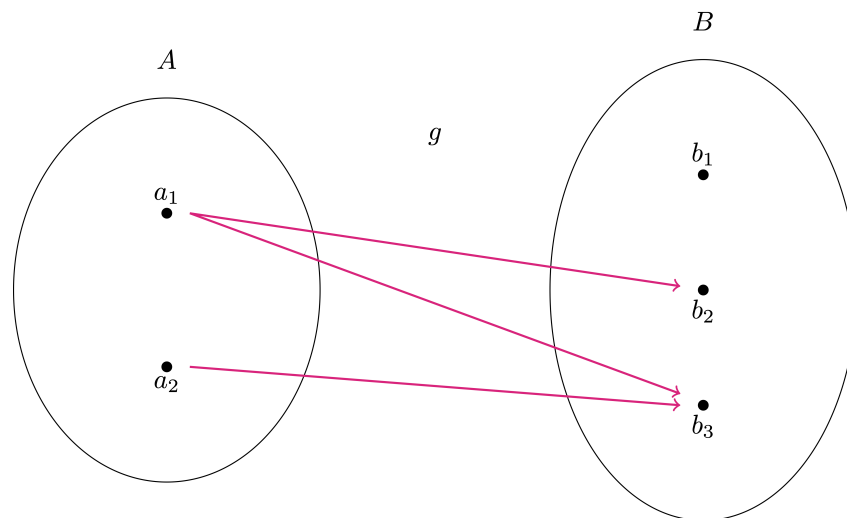
Figure 2.7: Schematic picture of the function g
