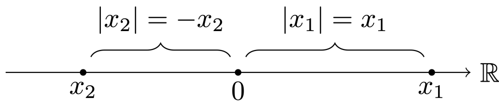
Figure 2.12: Geometric interpretation of |x|
