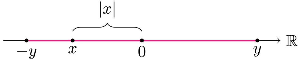
Figure 2.14: Geometric meaning of Lemma 2.35
