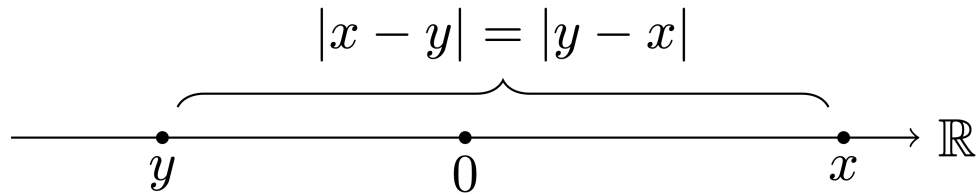
Figure 2.13: Geometric interpretation of |x - y|
